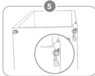
Unscrew bottom hinge. Then remove the adjustable feet from both side.
