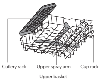
Upper basket
